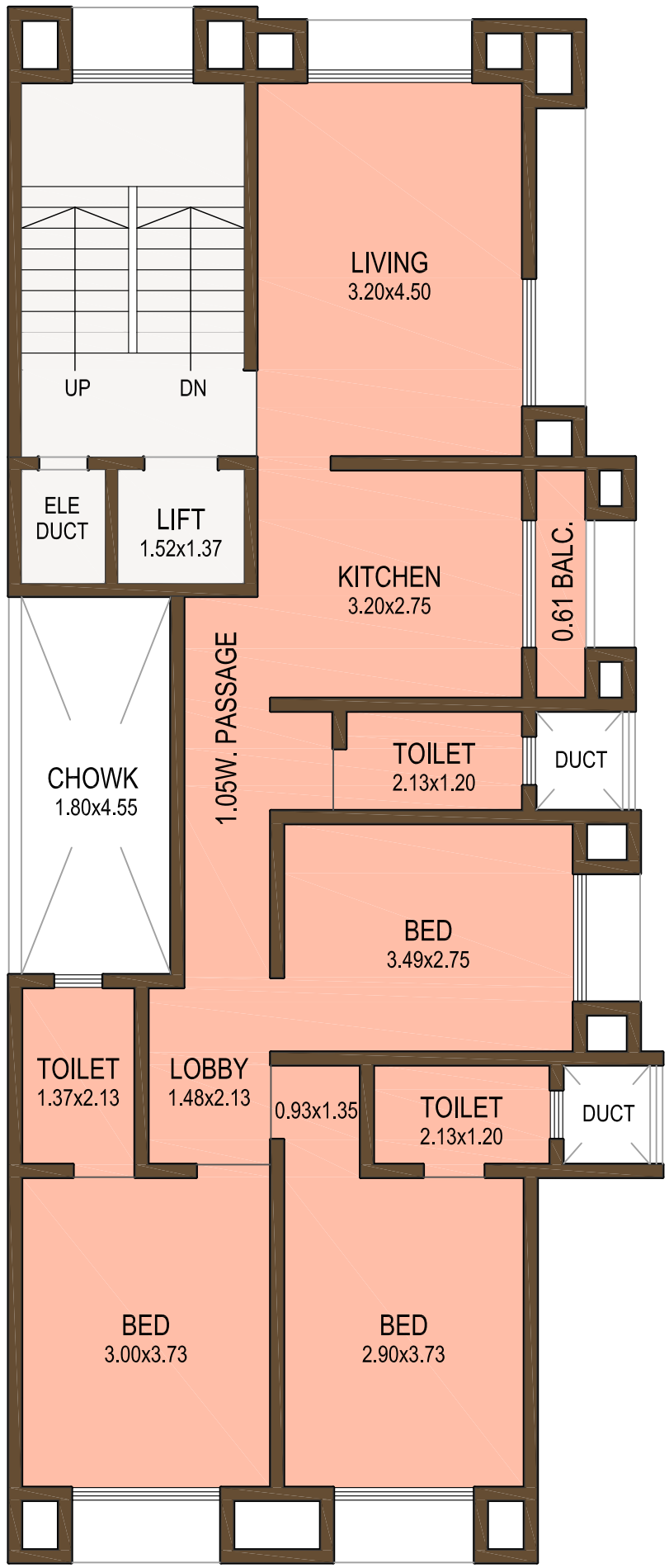
TYPICAL FLOOR PLAN
